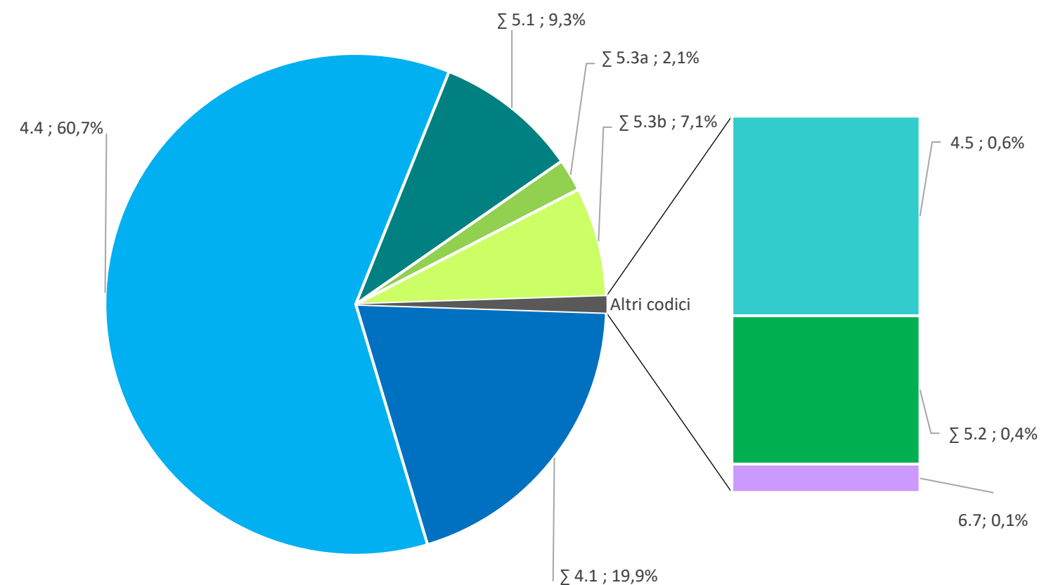
Pesticidi - FDM 2018
