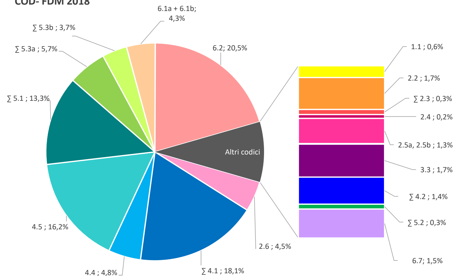
COD- FDM 2018
